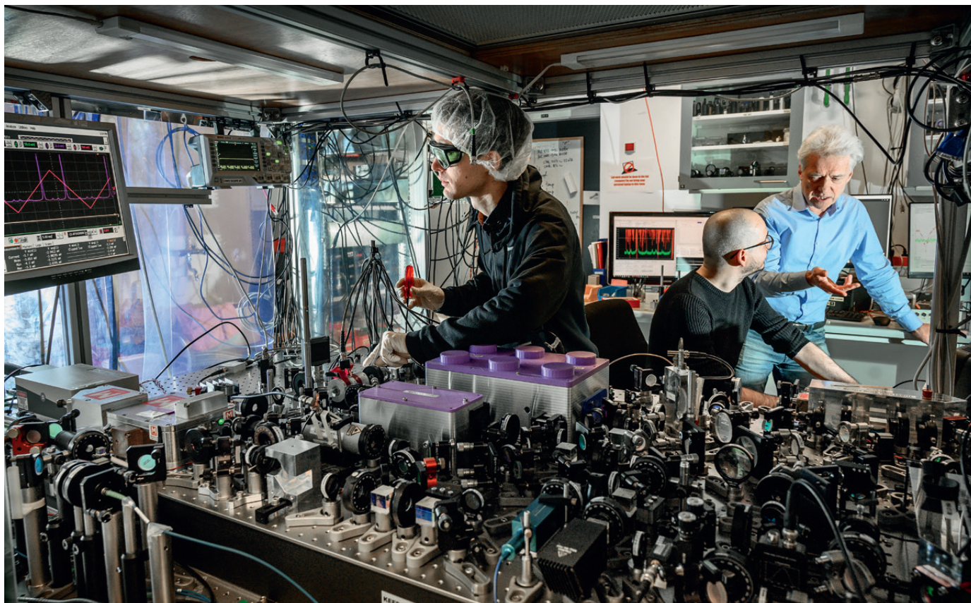
Experimental setup for quantum sensing by the group of professor Eugene Polzik (right). Here with PhD student Valerii Novikov (left) and postdoc Tulio Brito Brasil (center).
