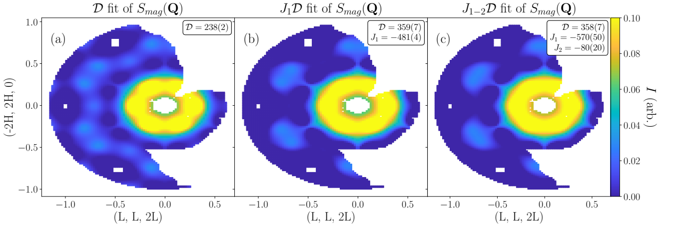
Figure 24: Same fits as shown in fig. 14 but without S_{mag}(\mathbf{Q}) . (a) \mathcal{D} fit, (b) J_1\mathcal{D} fit, and (c) J_{1-2}\mathcal{D} fit. Incident energy of E = 1.55 meV. Numbers in top right boxes show fitted interaction parameters and have units of mK. Number in parentheses indicate \pm uncertainty.
