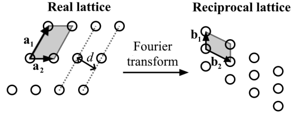
Figure 4: Left: 2D crystal lattice in real space with lattice vectors \mathbf{a}_1 and \mathbf{a}_2 . The shaded area is a primitive unit cell. The dotted lines show two lattice lines. Right: The corresponding primitive reciprocal lattice obtained from a Fourier transform with reciprocal lattice vectors \mathbf{b}_1 and \mathbf{b}_2 .
