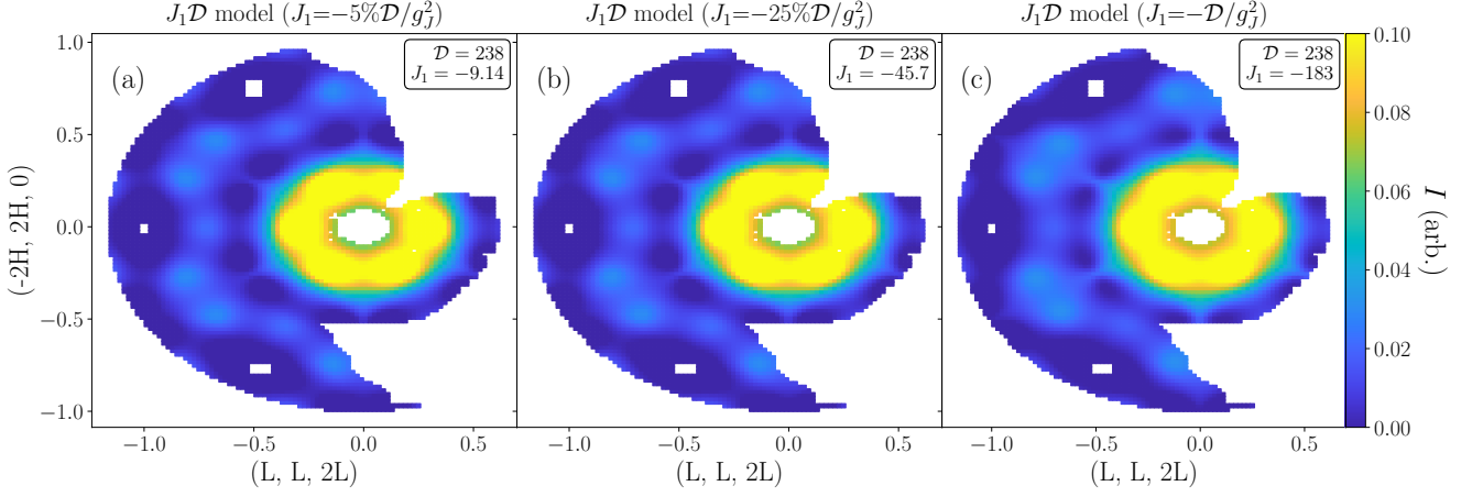
Figure 26: J_1\mathcal{D} models calculated with Spinteract for varying J_1 . (a) J_1 = -5\%\mathcal{D}/g_J^2 , (b) J_1 = -25\%\mathcal{D}/g_J^2 , and (c) J_1 = -\mathcal{D}/g_J^2 . Incident energy of E = 1.55 meV.
