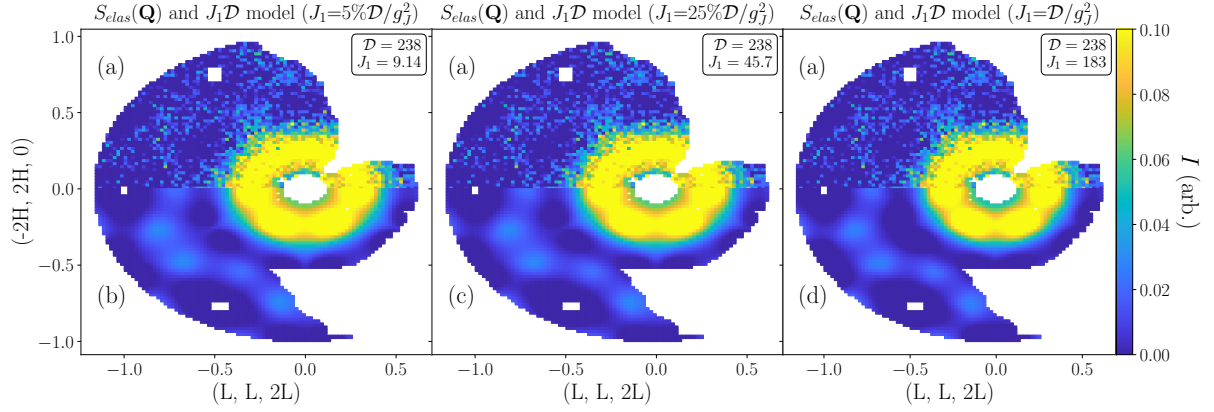
Figure 17: (a) S_{elas}(\mathbf{Q}) . J_1\mathcal{D} models calculated, not fitted, with Spinteract for varying J_1 with (b) J_1 = 5\%\mathcal{D}/g_J^2 , (c) J_1 = 25\%\mathcal{D}/g_J^2 , and (d) J_1 = \mathcal{D}/g_J^2 . Incident energy of E = 1.55 meV.
