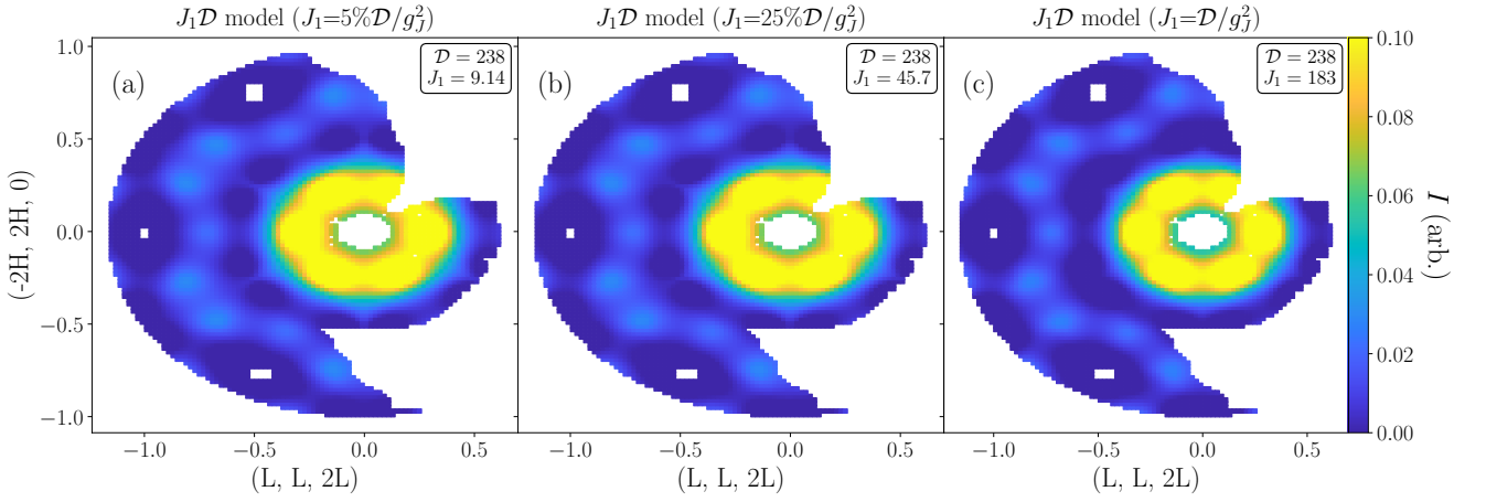
Figure 27: J_1\mathcal{D} models calculated with Spinteract for varying J_1 . (a) J_1 = 5\%\mathcal{D}/g_J^2 , (b) J_1 = 25\%\mathcal{D}/g_J^2 , and (c) J_1 = \mathcal{D}/g_J^2 . Incident energy of E = 1.55 meV.
