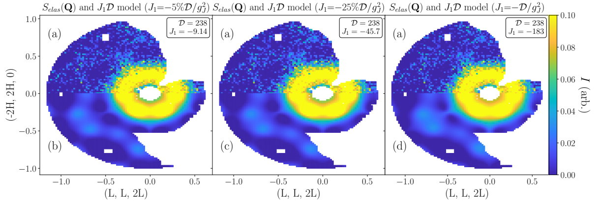
Figure 18: (a) S_{elas}(\mathbf{Q}) . J_1\mathcal{D} models calculated, not fitted, with Spinteract for varying J_1 with (b) J_1 = -5\%\mathcal{D}/g_J^2 , (c) J_1 = -25\%\mathcal{D}/g_J^2 , and (d) J_1 = -\mathcal{D}/g_J^2 . Incident energy of E = 1.55 meV.
