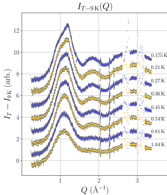
Figure 6: Neutron diffraction data from [10], I_{T-9K}(Q) , for GGG between 0.175 - 1.04 K with grey uncertainties. 9 K data subtracted. An arbitrary spacing of 1.2 is added between each curve for clarity. Nuclear Bragg peaks have been removed in the two gaps near Q \approx 3 \text{ \AA}^{-1} .
