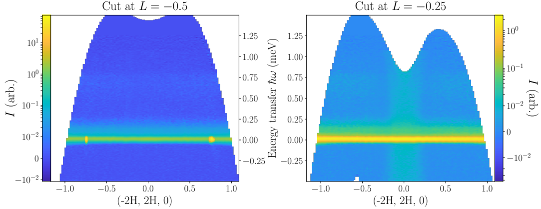
Figure 9: Cuts at different values of L in the data with E = 1.55 meV. Left: L = -0.5 . Right: L = -0.25 . Positive values of \hbar\omega indicate energy transferred to the sample while negative values indicate energy absorbed by the neutron. The T = 13 K data has been subtracted. Both graphs have their own logarithmic colormaps.
